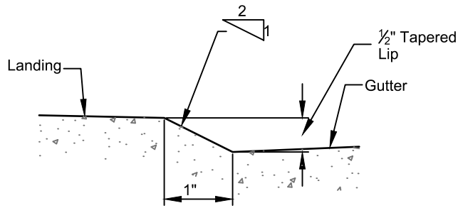
LIP DETAIL
