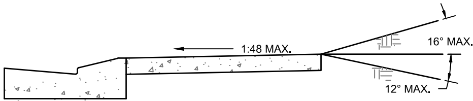
TYPICAL DRIVEWAY APPROACH
