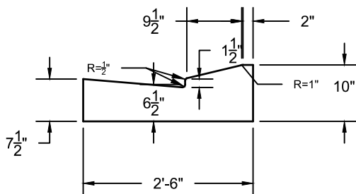
MOUNTABLE CURB DETAIL
