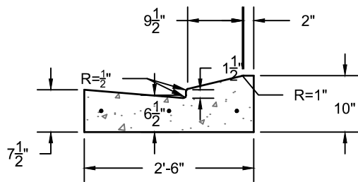
MOUNTABLE CURB DETAIL
